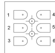
Socket view of screw terminals
