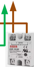
SSR Bed heater
