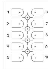
Socket view of screw terminals
